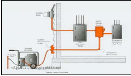
Integrated System – Portable Generator Installation
